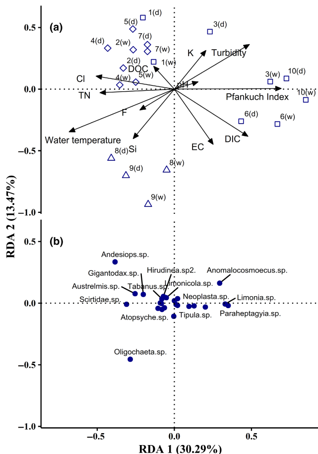
FIGURE 5 Redundancy analysis (RDA) ordination diagrams of (a) environmental variables and sites, and (b) macroinvertebrate taxa. DIC, dissolved inorganic carbon; DOC, dissolved organic carbon; EC, electrical conductivity; TN, total nitrogen. Numbers correspond to sites labelled in Figure 1; letters in parentheses represent sample season; d, dry; w, wet. Shapes represent GCC categories (Low: \triangle , Medium: \diamond , High: \square ).
