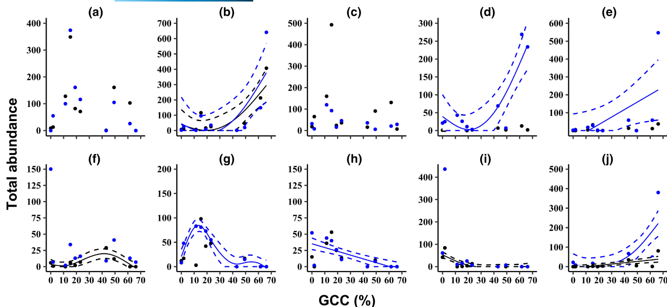
FIGURE 4 Relationships between glacier cover in a catchment (GCC) and mean abundance of selected taxa: (a) Andesiops sp., (b) Anomalocosmoecus sp., (c) Gigantodax sp., (d) Orthocladinae sp., (e) Paraheptagya sp., (f) Ceratopogoninae sp., (g) Scirtidae sp., (h) Austrelmis sp., (i) Oligochaeta sp., and (j) Limonia sp. The colour of lines represents dry (black) and wet (blue) seasons. Lines represent of best fit in GAM models except (e) and (h) in wet season, and (j) in dry season, which represent generalized linear models. Dashed lines represent 95% confidence intervals.
